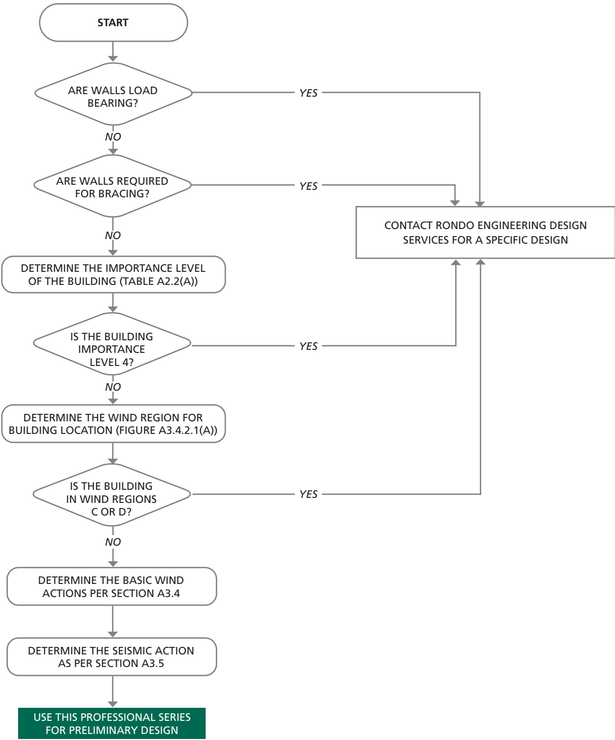
■ FIGURE C1.2(A) - APPLICABILITY OF PROFESSIONAL SERIES FOR PRELIMINARY DESIGN
